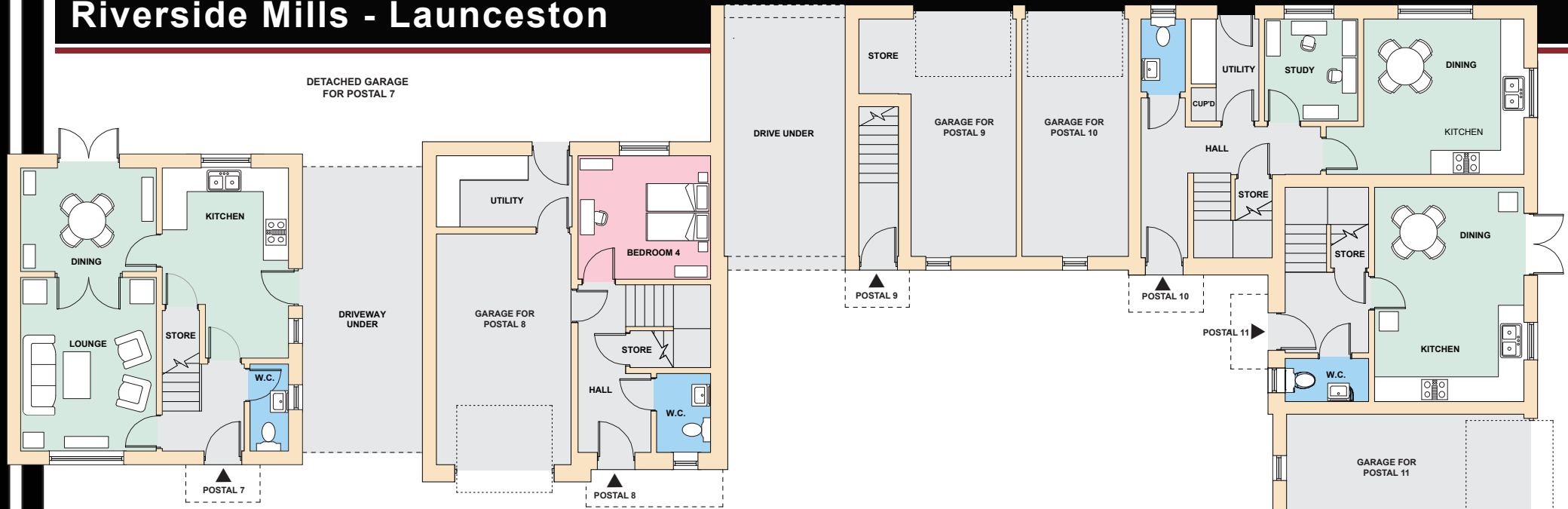
Ground floor layouts - postal no's 7, 8, 9, 11 and 12
